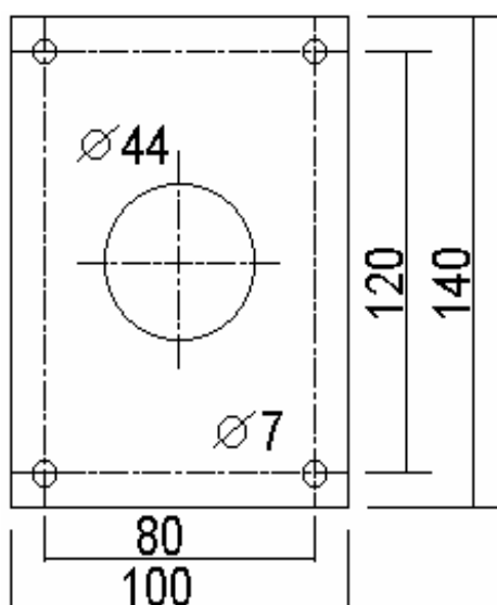
ground plate
